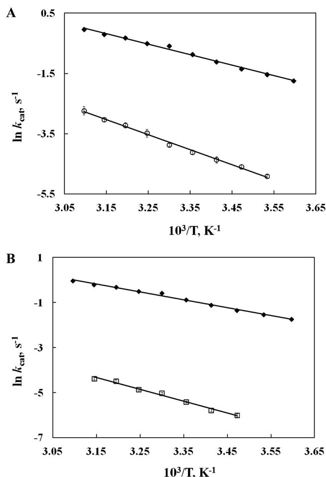
Figure 2. (A) Arrhenius plots of SLO-1 double mutants for k_{\text{cat}} with protio-LA. Data points for Ile553Ala/Leu754Ala (◆) from 5 to 50 °C and Leu546Ala/Leu754Ala (○) from 10 to 50 °C in 0.1 M borate (pH 9.0). (B) Impact of substrate deuteration on the k_{\text{cat}} for the Ile553Ala/Leu754Ala SLO-1 double mutant. Data points for 11,11- d_2 -LA (□) from 15 to 45 °C in 0.1 M borate (pH 9.0). For comparison, the data points for protio-LA (◆) from 5 to 50 °C are also shown.
